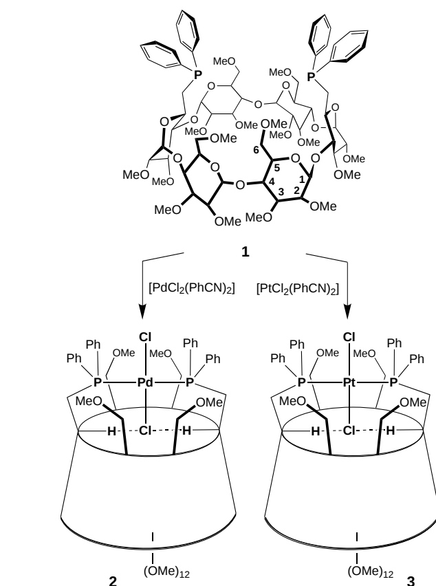
Scheme 1. trans -Binding behavior of 1 . Synthesis of 2 and 3 .
